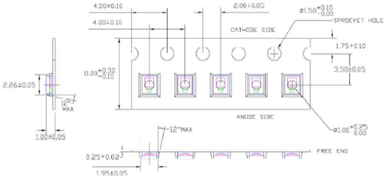
Figure 16. Tape dimensions.
