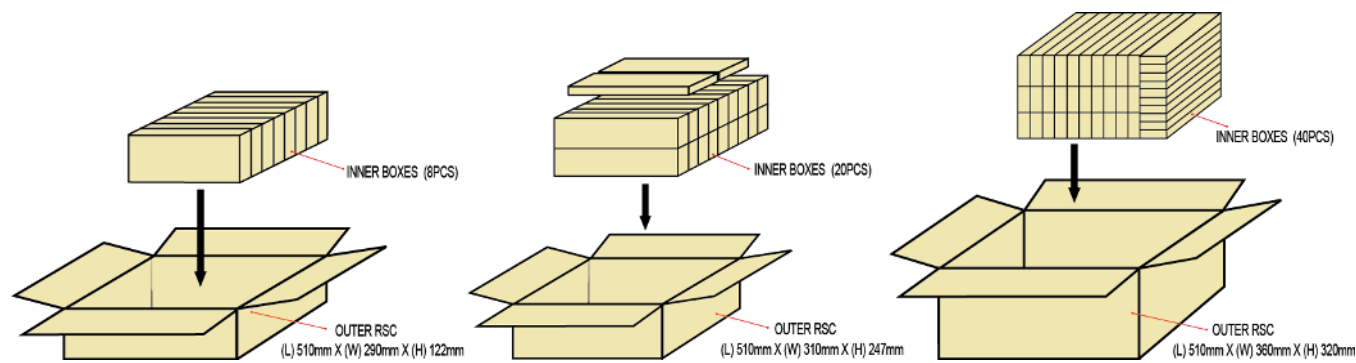
Figure 13. Dimensions for outer box packaging for LUXEON CoB with FreshFocus Technology.
