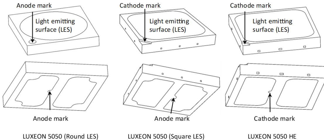
Figure 1. Package rendering of the LUXEON 5050 emitter.
