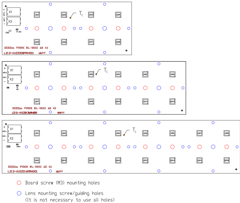
Figure 3: T_c locations, board and lens mounting screw/guiding holes for all LUXEON XR-5050 Round configurations.
