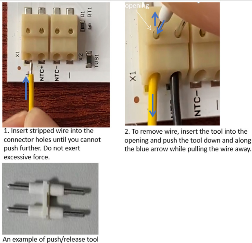
Figure 6: Inserting and removing wire from connector #3.
