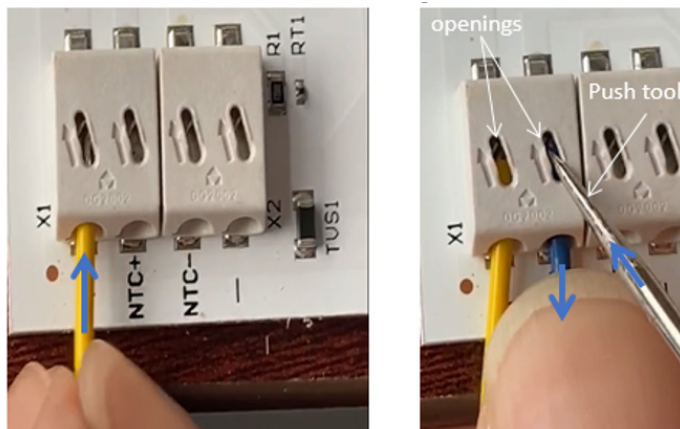
1. Insert stripped wire into the connector holes until you cannot push further. Do not exert excessive force.
