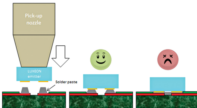
Figure 31. A proper starting point for the mounting z-height of LUXEON emitter is \frac{1}{3} rd of the stencil thickness with reference to the top of the stencil paste, i.e. the collet should be in an under-travel position. Center picture shows the optimum result for the collet height setting. Right picture shows over-travel position and may result in bridging of the solder paste on adjacent pads prior to reflow.
