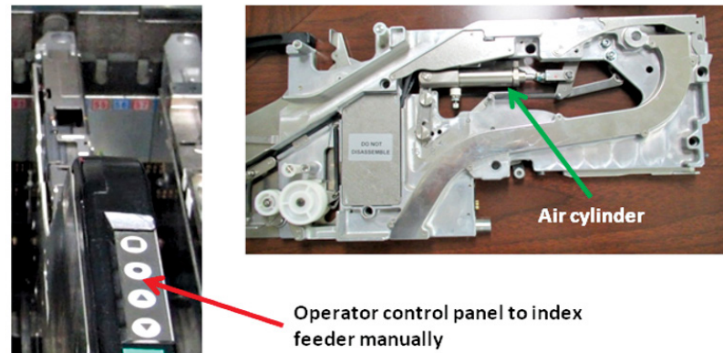
Figure 25. Examples of an electric feeder (left) and a pneumatic feeder (right) which are typically used in pick and place machines to advance the tape with LEDs.
