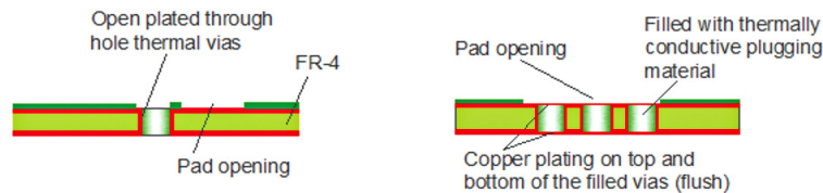
Figure 6. Left picture shows a cross section of an open via with plated through hole design with one pad opening where the LED pad is soldered onto. Right picture shows a cross section of a filled and cap via design with one pad opening. One of the LED pads is then soldered on top of the flush area where the filled and capped vias are underneath it to create direct thermal path connection between LED and bottom of PCB.
