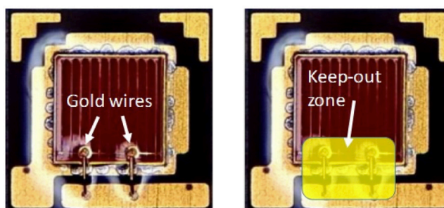
Figure 3b. Keep-out zone when handling LUXEON CZ AlInGaP.
