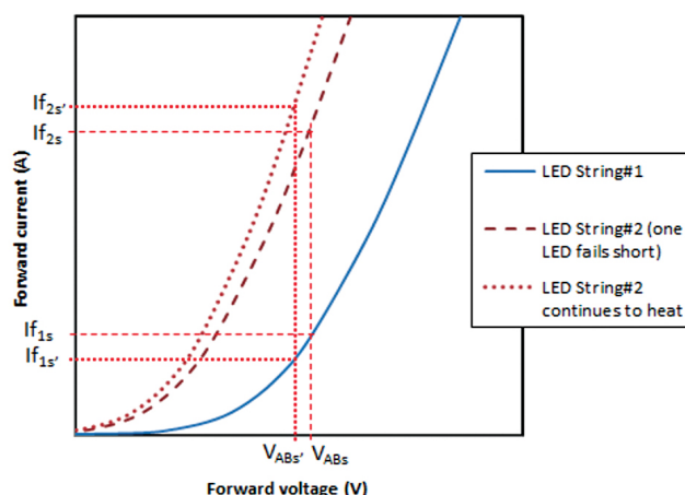
Figure 11. Thermal run-away on LED string #2 due to increase current (therefore heating) will further shift its current-voltage curve to the left and increase the LED string#2 current from I_{f_{2s}} to I_{f_{2s'}} .
