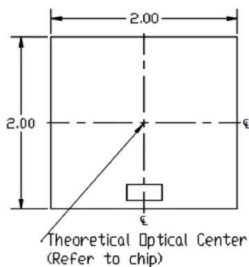
Figure 2. Optical center. All dimensions in millimeters.
