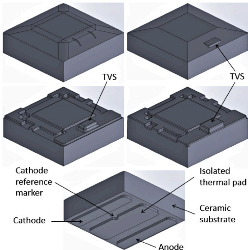
Figure 1. Image rendering of LUXEON CZ emitter. From top left (clockwise) represents LUXEON CZ with AlInGaP chip, PCAmber, white/mint and InGaN direct colors. Bottom most picture shows the pad design for all the four configurations.
