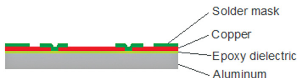
Figure 5. MCPCB typical cross section of the three-pad openings with aluminum substrate.
