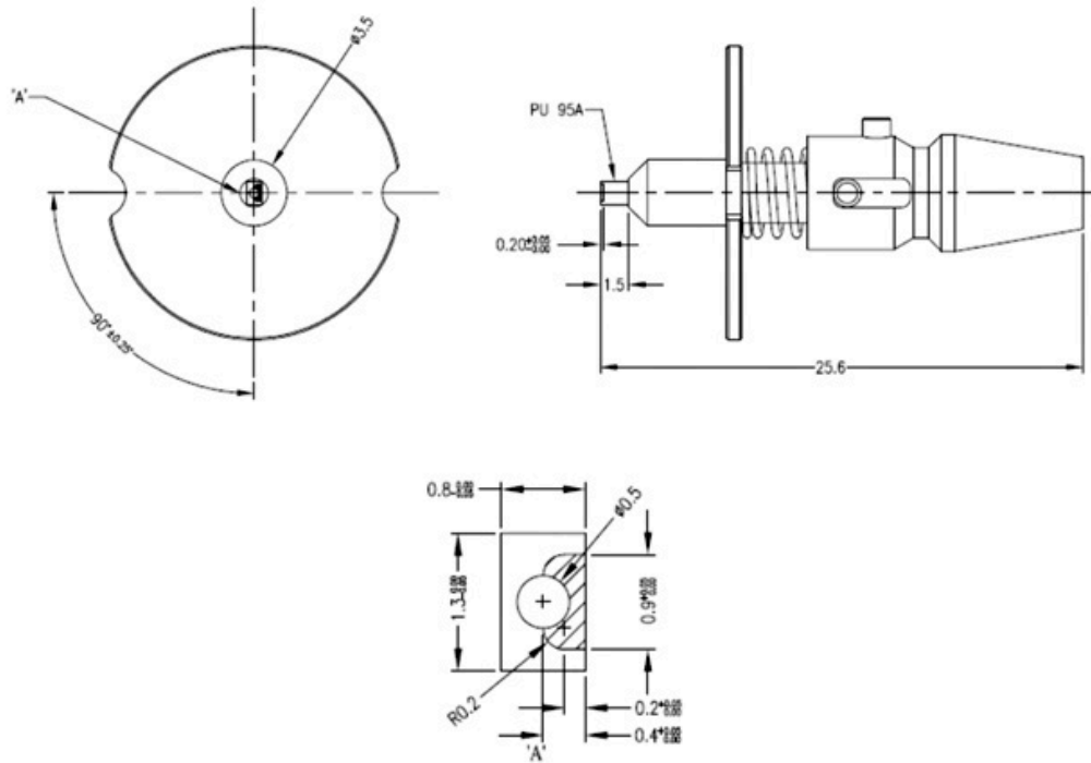
Figure 19. Nozzle design for LUXEON CZ AlInGaP using Samsung SM421 (part number: SAM-0567 / 17, drawing number: 14483 from Ching Yi Technology Pte Ltd, http://www.chingyi.com.sg ). All dimensions are in millimeters.
