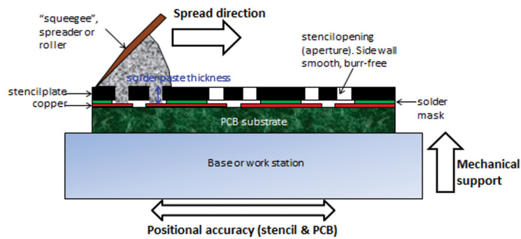
Figure 12. Stencil printing process.
