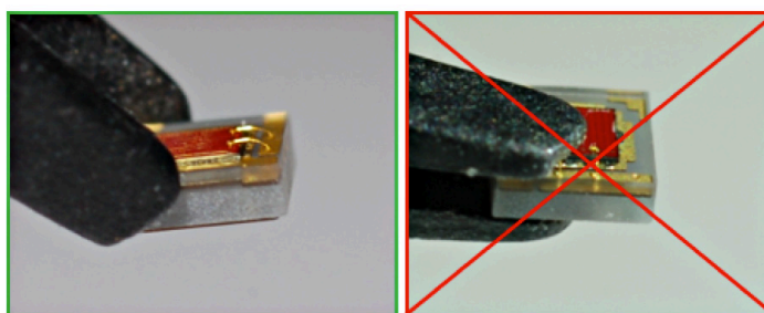
Figure 3a. Correct handling (left) and incorrect handling (right) of LUXEON CZ.
