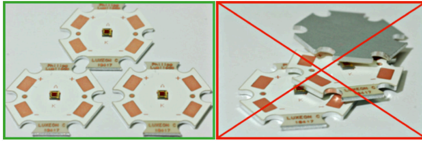
Figure 3c. Correct placement of assembled board (left) and incorrect stacking of assembled boards (right).
