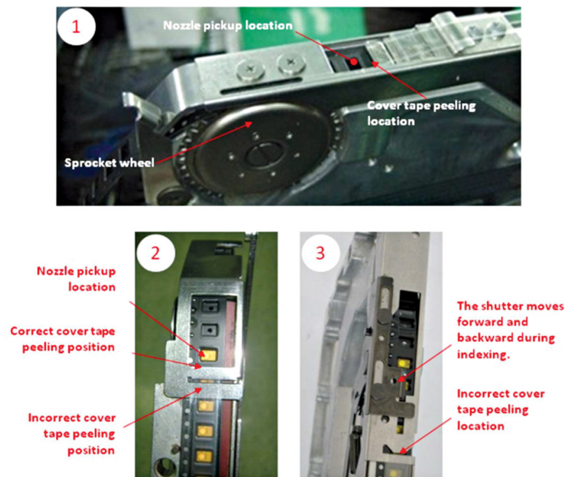
Figure 26. Three representative feeder designs. Feeder 1 does not require any modification. Feeder 2 requires the cover tape peeling position to be shifted. Feeder 3 requires the shutter to be removed before the cover tape peeling position can be adjusted.
