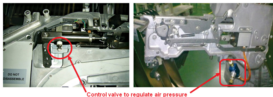
Figure 29. Pneumatic feeder with integrated air pressure control valve (left) and pneumatic feeder with air pressure control valve installed afterwards (right).
