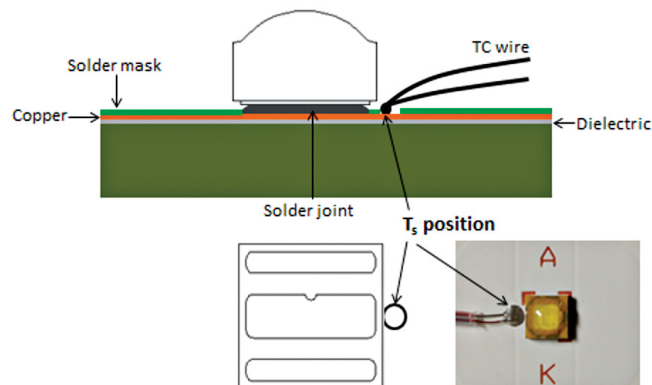
Figure 33. T_s location for LUXEON CZ mounted on PCB. Place the TC wire as close as possible to the LUXEON CZ thermal pad (shown in the drawing is LUXEON C with similar package footprint as LUXEON CZ).
