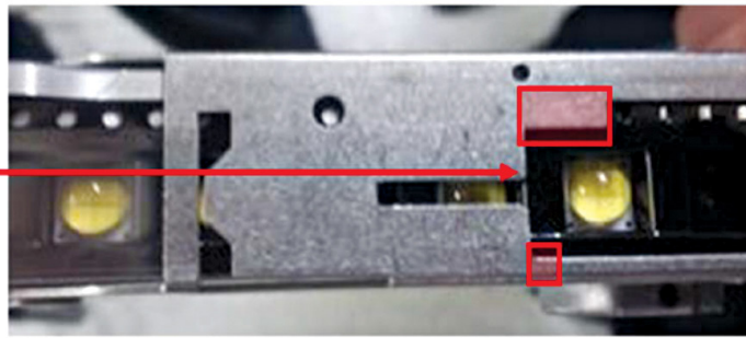
Figure 30. The cover tape peeling location in this feeder needs to be widened so that the cover tape can be peeled off without any obstruction.
