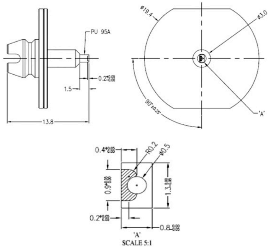
Figure 21. Nozzle design for LUXEON CZ AlInGaP using Panasonic CM402 (part number: KME-0566 / 17, drawing number: 14482 from Ching Yi Technology Pte Ltd, http://www.chingyi.com.sg ). All dimensions are in millimeters.
