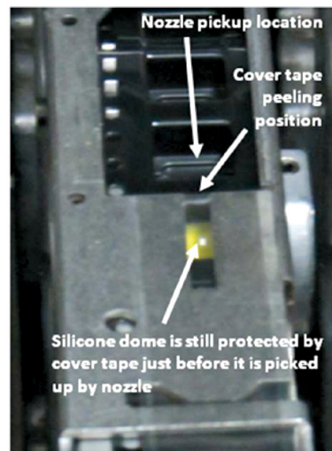
Figure 28. Example of a modified feeder which protects the silicone dome prior to pickup.
