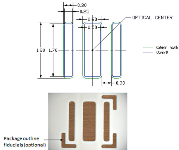
Figure 4. LUXEON CZ PCB footprint (top). Actual LUXEON CZ PCB with white solder mask and optional package outline fiducials (bottom). All dimensions in millimeters.
