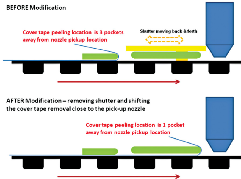
Figure 27. Illustration of the general principle behind the feeder modification.
