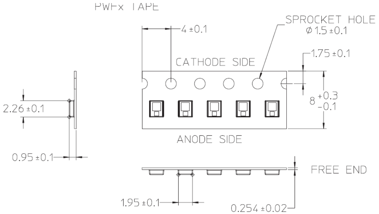
Figure 16. Tape dimensions.
