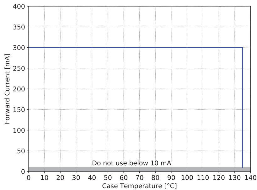
Figure 6. Maximum forward current vs. case temperature for SignalSure 140
