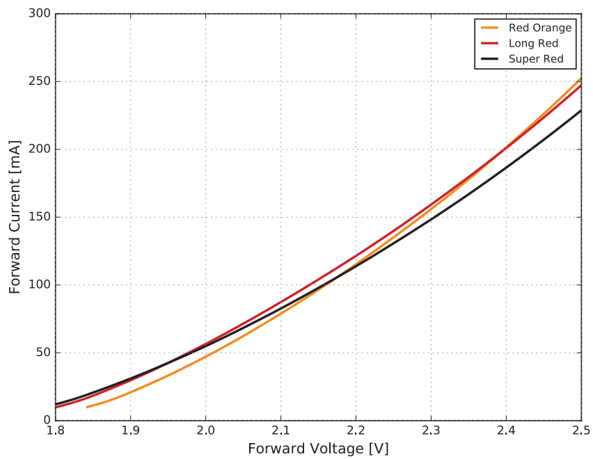
Figure 4a. Typical forward current vs. forward voltage for SignalSure 140 at T_j = 25\text{ }^{\circ}\text{C}
