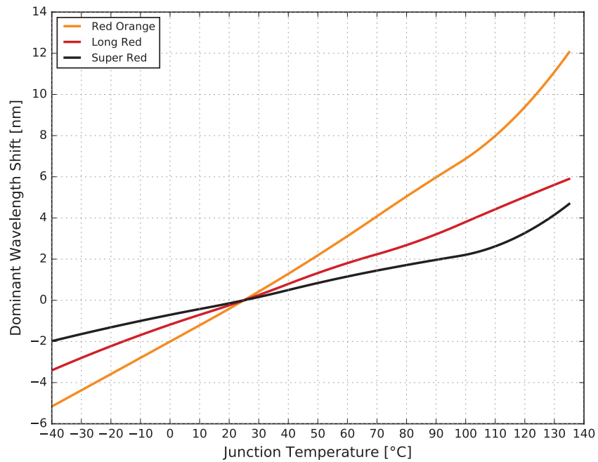
Figure 1b. Typical wavelength shift vs junction temperature for SignalSure 140 at 20 ms MP, 140 mA, T_j = 25\text{ °C}
