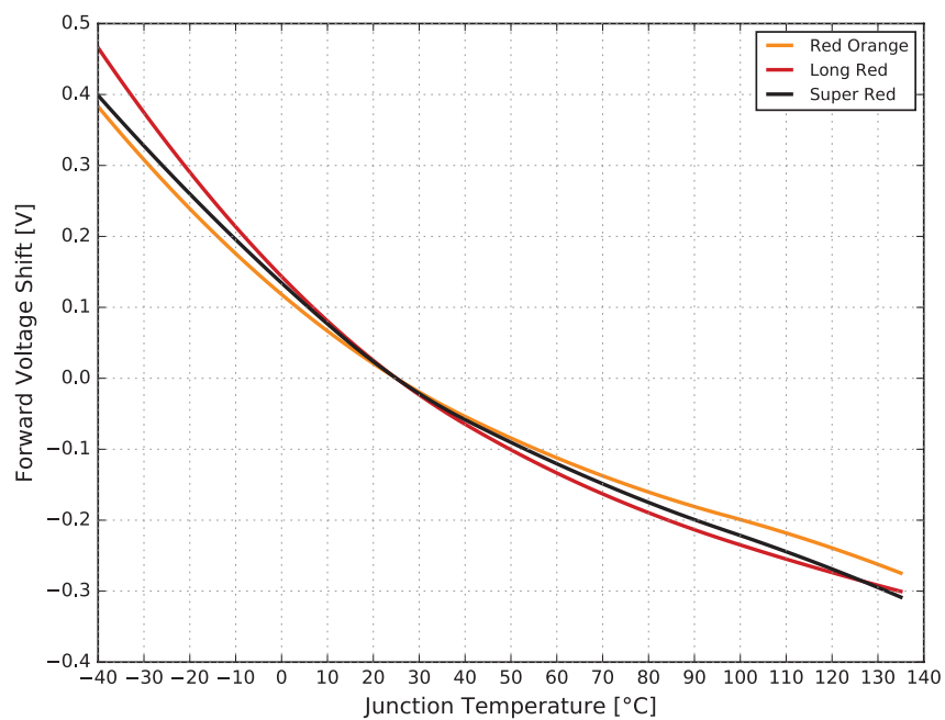
Figure 4b. Typical forward voltage shift vs. junction temperature for SignalSure 140 at 20 ms MP, specified test current
