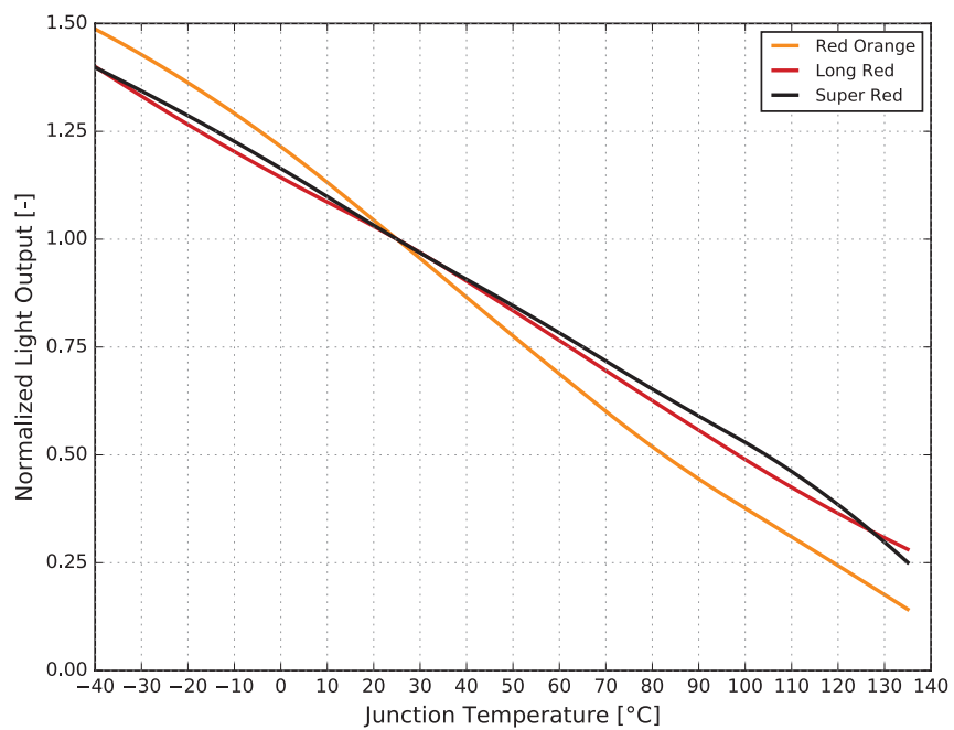
Figure 2. Typical normalized light output vs. junction temperature for SignalSure 140 at 20 ms MP, 140 mA
