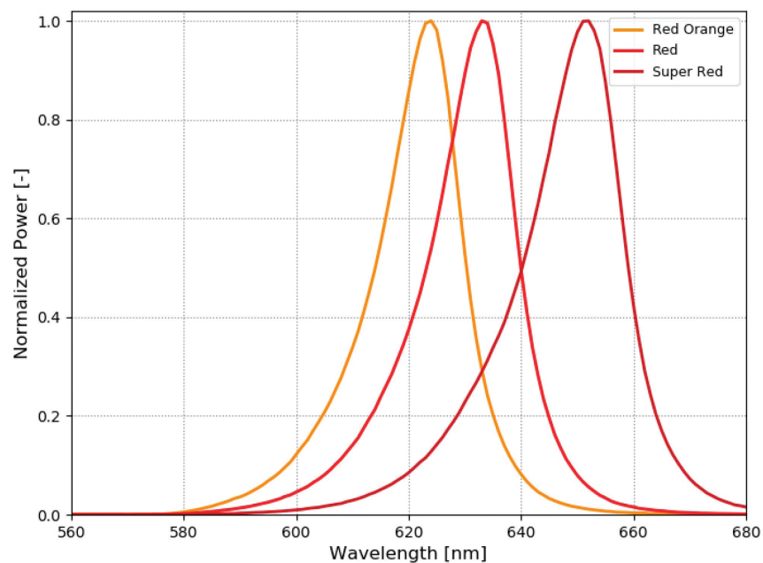
Figure 1a. Typical normalized power vs. wavelength for SignalSure 140 at 20 ms MP, 140 mA, T j = 25 °C
