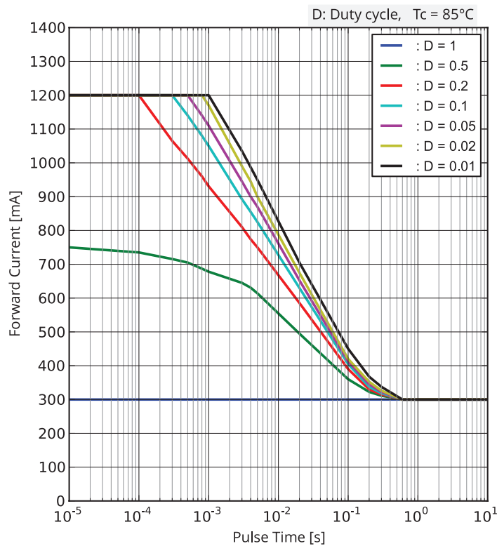
Figure 7. Permissible pulse handling capability for SignalSure 140
