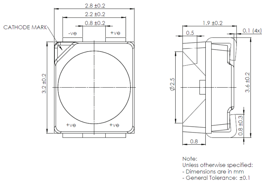
Figure 8. Mechanical dimensions for SignalSure 140
