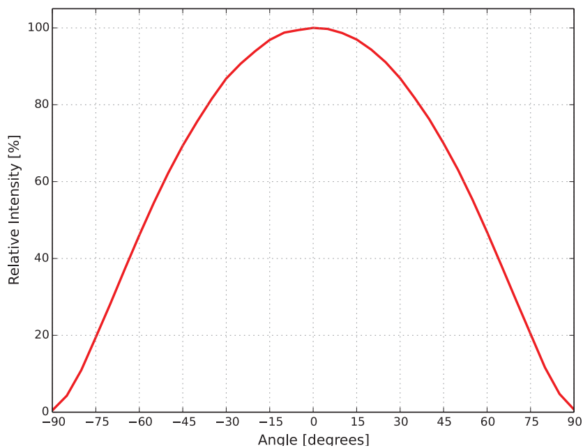
Figure 5. Typical radiation pattern for SignalSure 140 at 20 ms MP, 140 mA
