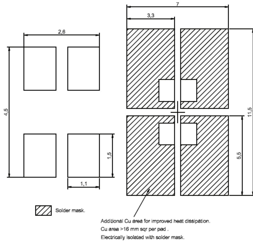
Figure 10. Recommended solder pad layout for SignalSure 140
