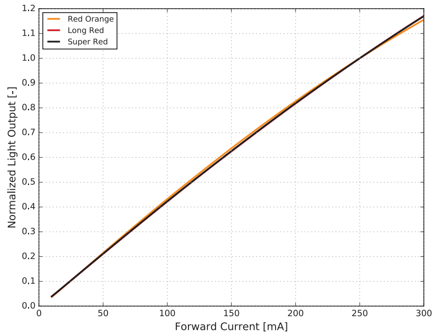
Figure 3. Typical normalized light output vs. forward current for SignalSure 140 at T_j = 25\text{ }^{\circ}\text{C}
