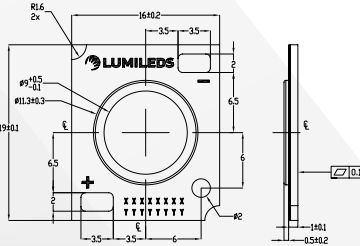
L2C5-xxHG1202E0900, L2C5-xxHG1203E0900
