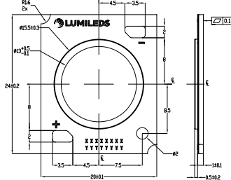
L2C5-xxHG1204E1300, L2C5-xxHG1205E1300
